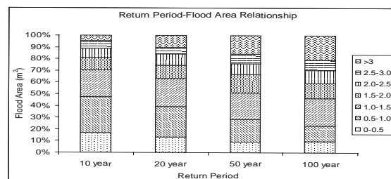
Figure 4: Relationship between return period and flood area.
